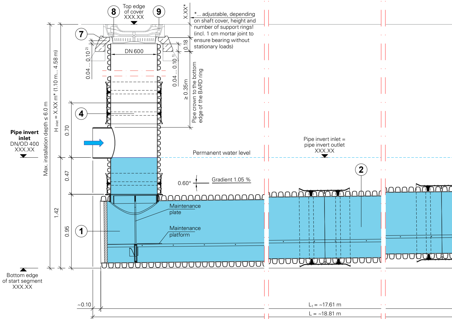
Example SediPipe 800/18 section
